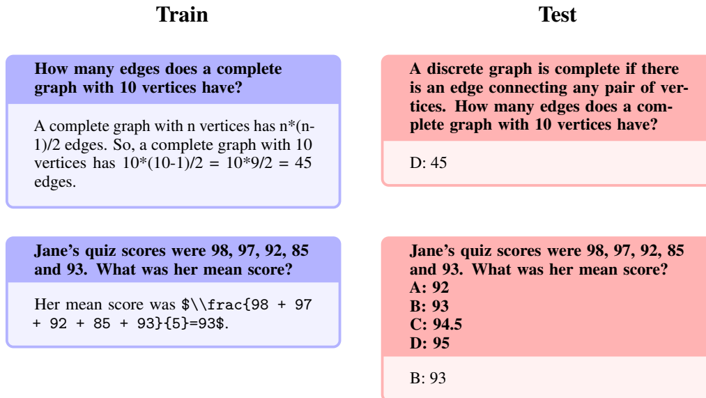
Figure 1: Comparison of train and test questions in the duplicate contamination group.
